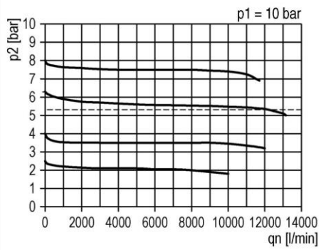
flow characteristic
